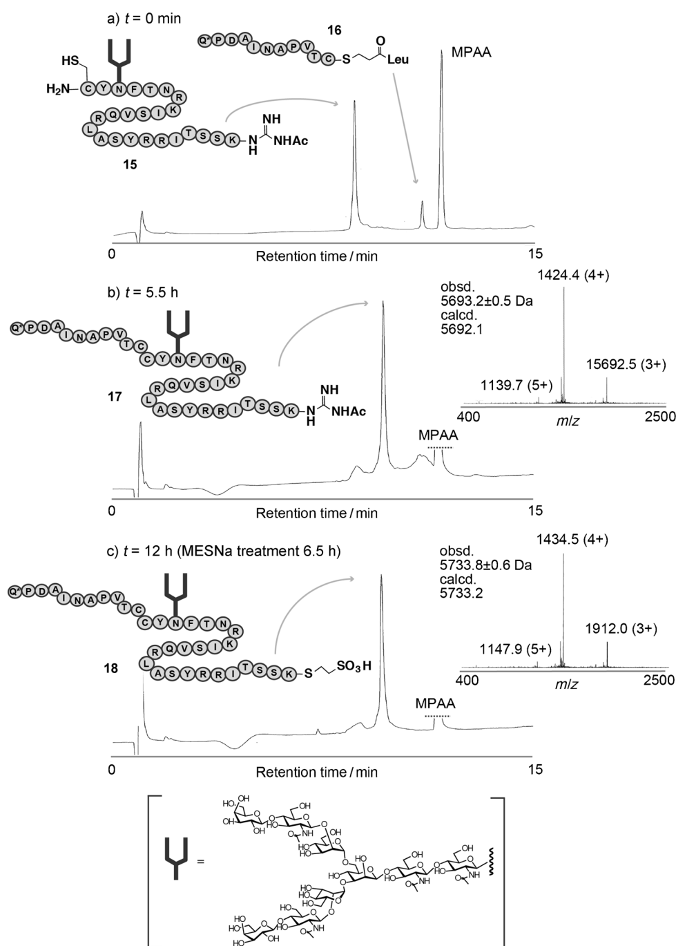
Figure 2. KCL between the peptide MPAL thioester and Cys-glycopeptidyl- N -acetylguanidine. The reaction was monitored by RP-HPLC: a) t = 0 min, b) t = 5.5 h, and c) t = 12 h in the total reaction time. After completion of the KCL (b) t = 5.5 h, MESNa was added to the reaction (10% wt/wt) and the 35-aa glycopeptidyl- N -acetylguanidine 17 was efficiently converted into the corresponding MESNa thioester 18 in 6.5 h (c), total reaction time was 12 h. Each inset is the ESI mass spectrum of each peak. Q* = pyroglutamine, Q = Gln = glutamine, P = Pro = proline, D = Asp = aspartic acid, I = Ile = isoleucine, T = Thr = threonine.
